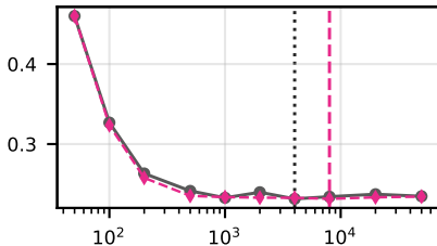
Appliances / PatchTST
