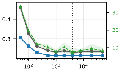
Appliances / PatchTST
