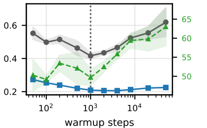
Appliances / PatchTST
