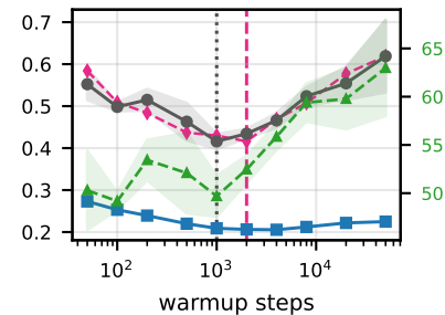
Appliances / PatchTST
