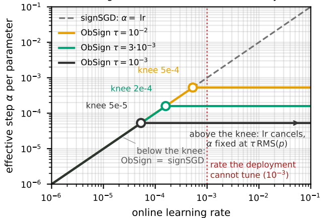
(A) the effective step \alpha = \min(\text{lr}, \tau \text{RMS}(p)) has two regimes, and the knee is where they meet
