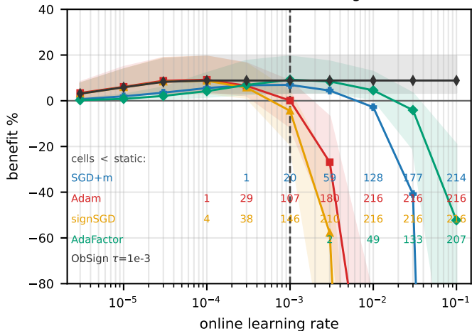
(A) benefit vs online learning rate
