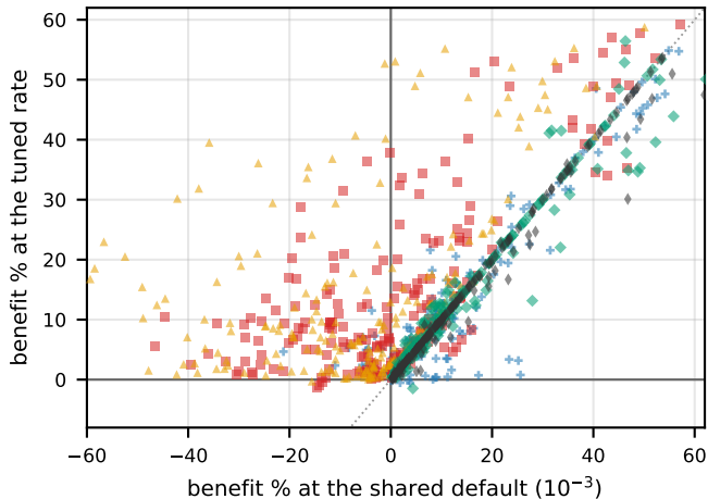
(B) benefit at the default vs at the tuned rate
