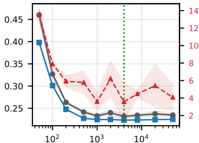
Appliances / PatchTST
