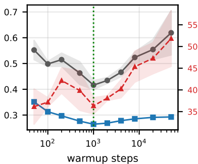
Appliances / PatchTST
