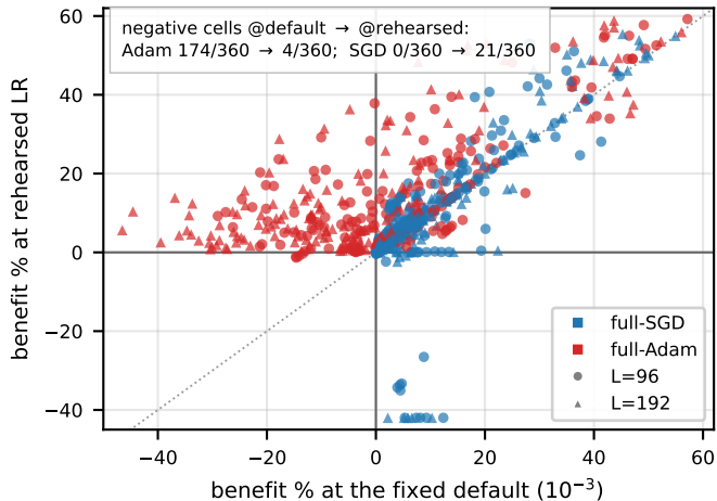
(B) rehearsal rescues Adam; can sink SGD (bottom edge)
