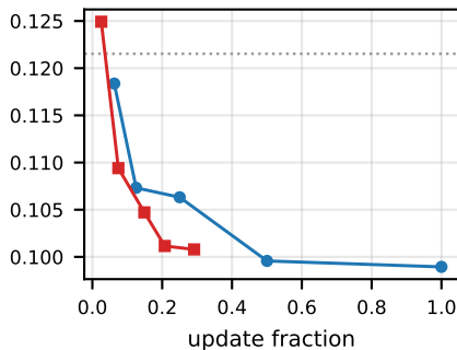
ETTh2 · full-Adam (drift +4.4%)
