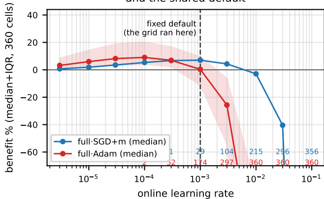
(A) Empirical nonnegative-benefit ranges and the shared default
