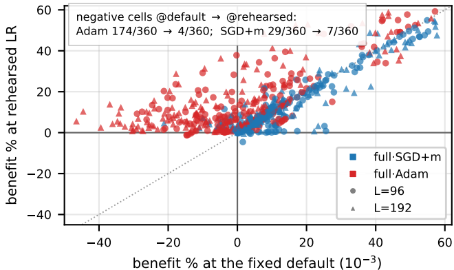
(B) Validation-based rehearsal substantially reduces Adam's below-static cells
