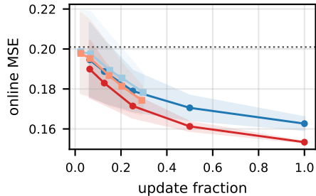
ETTh2 ( \Delta vs periodic: -1.1% / -2.8%)
