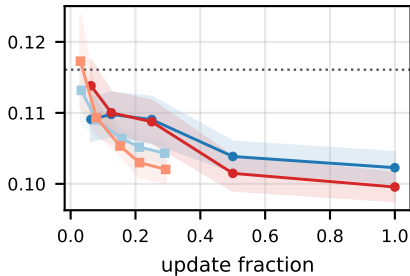
ETTh2 ( \Delta vs periodic: +2.6% / +4.5%)
