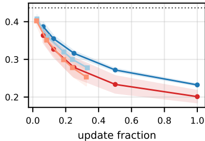
Appliances ( \Delta vs periodic: +5.6% / +1.9%)
