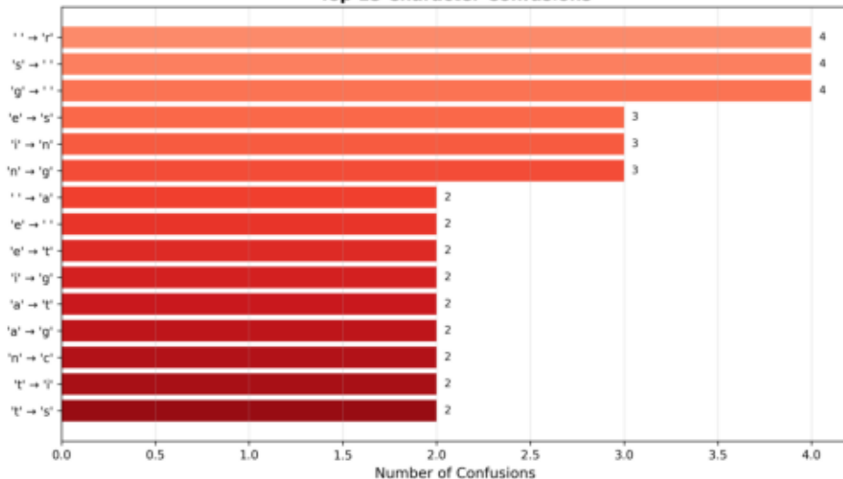
Top 15 Character Confusions
