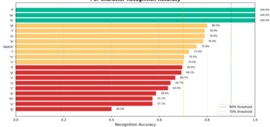
Per-Character Recognition Accuracy
