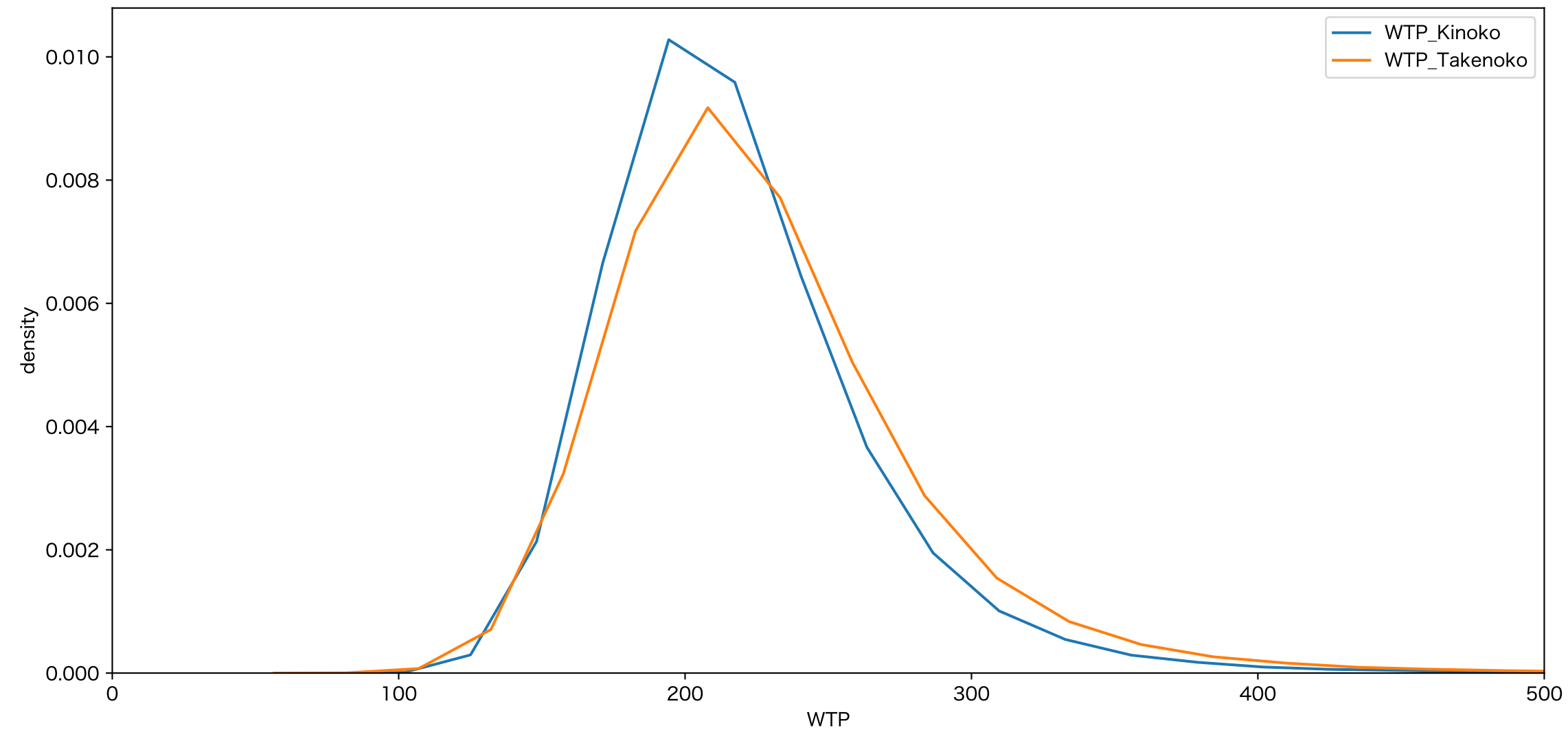
Distribution of WTP
