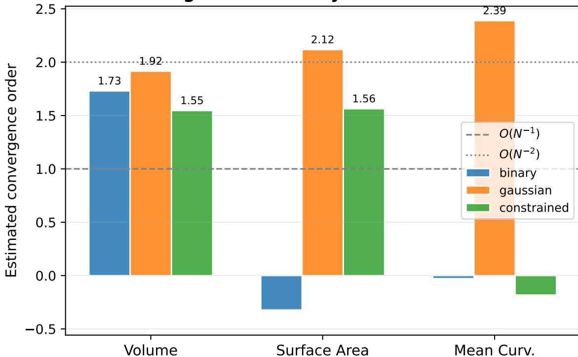
Convergence Orders by Method and Metric
