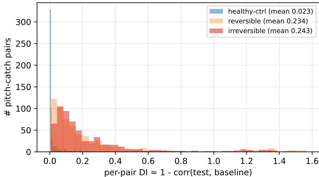
(a) damage index distributions @180 kHz [R] healthy-control = false-alarm floor
