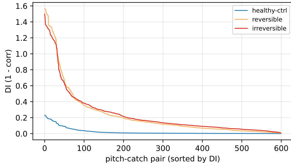
(b) sorted DI: damage lifts the whole curve above the healthy floor [R]
