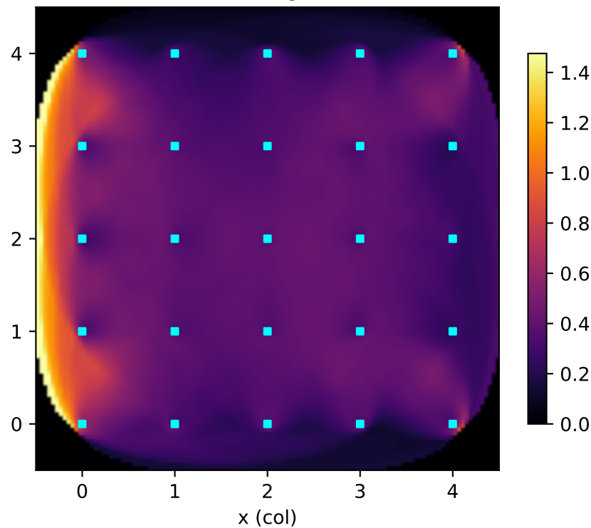
(B) RAPID damage image, irreversible [R/U] (assumed uniform grid coords [U])
