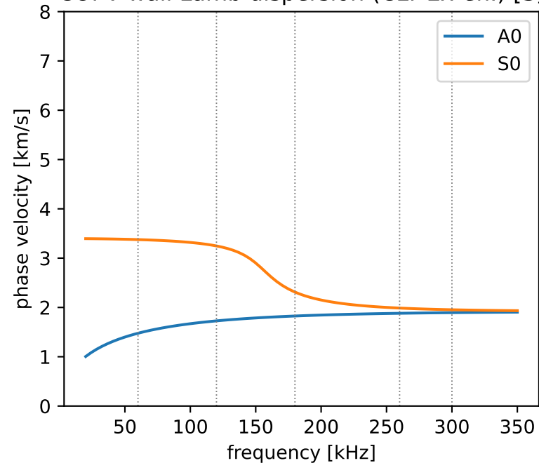
COPV wall Lamb dispersion (CLT Ex-eff.) [S]
