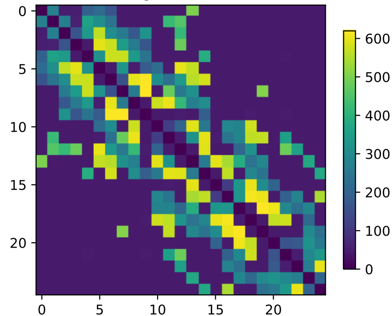
(a) PZT-PZT distance from ToF [R] mm, v_g=2900 m/s [U]
