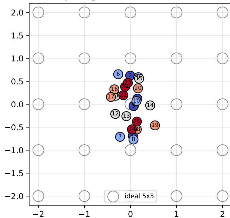
(c) unrolled vs ideal 5x5 [R] spacing~68 mm, RMSE=1.77
