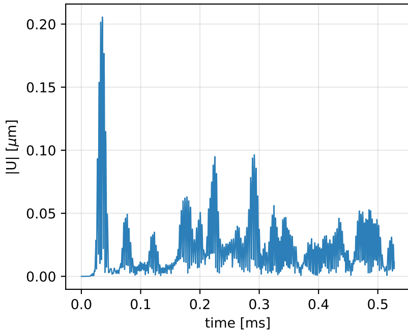
(b) representative RX packet @180 kHz (B1.87159)
