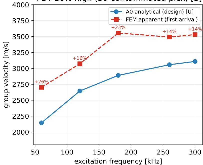
(a) A0 dispersion: FEM tracks trend, +14-26% high (S0-contaminated pick) [S]
