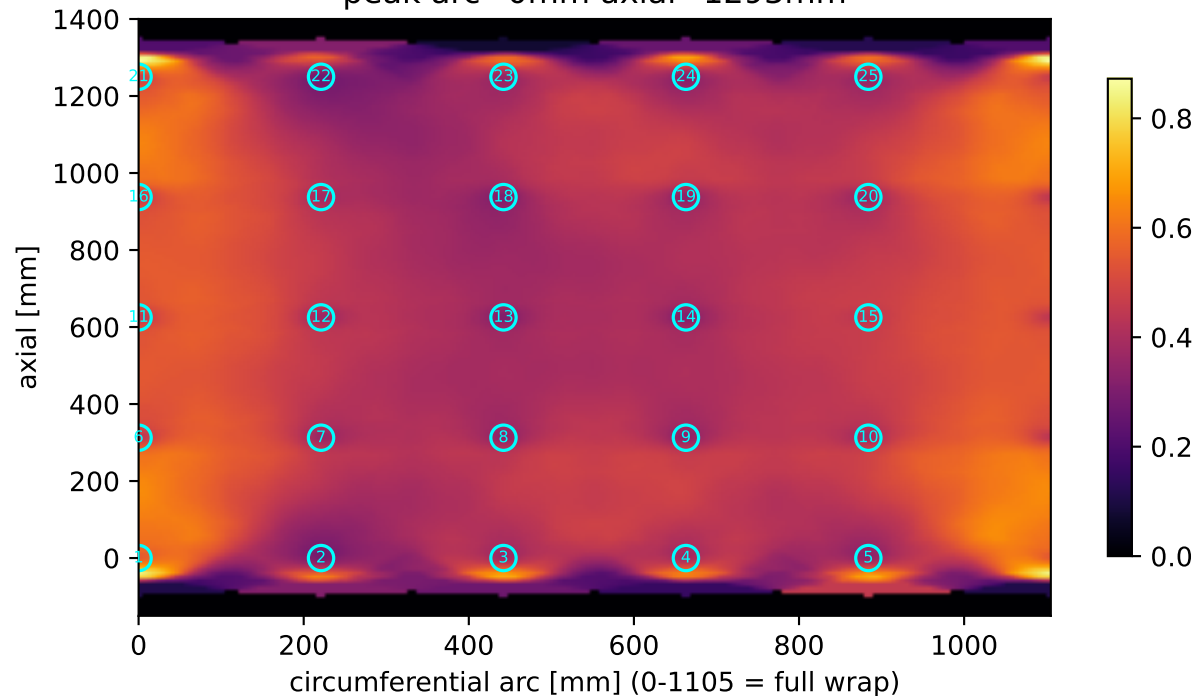
(B) RAPID damage image on TRUE unrolled cylinder [R] peak arc=0mm axial=1293mm
