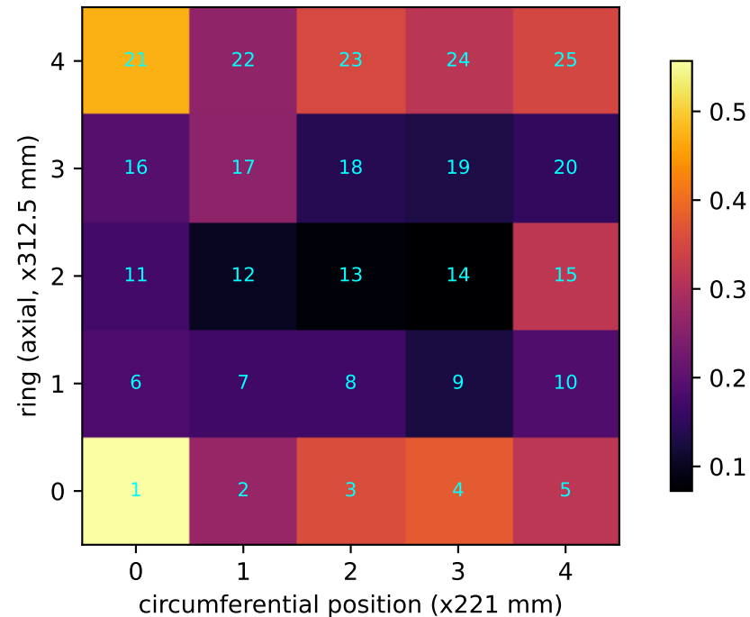
(A) per-PZT damage involvement [R] (true 5x5 ring x circumference)
