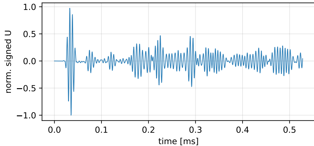
(b) SIM Abaqus RX 180 kHz 90deg sector [S/U] (B1.87159)
