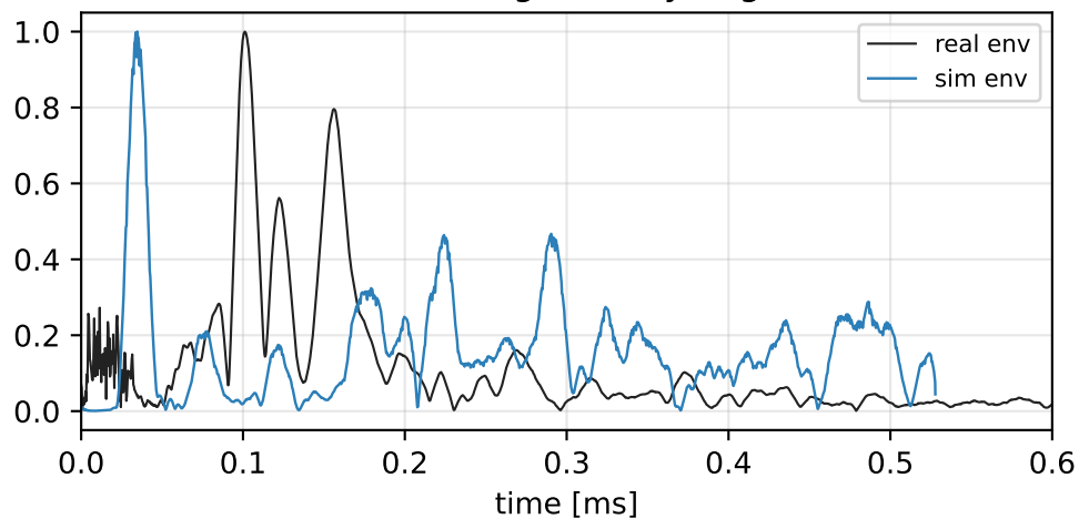
(c) packet envelope, first 0.6 ms (time axes NOT geometry-aligned [U])
