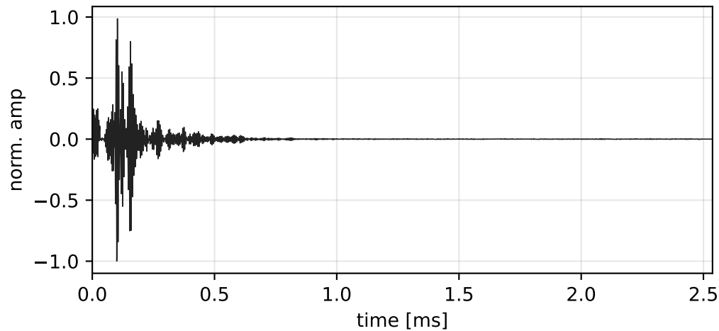
(a) REAL BAM RX TX1->RX2 180 kHz 700bar T25 [R]
