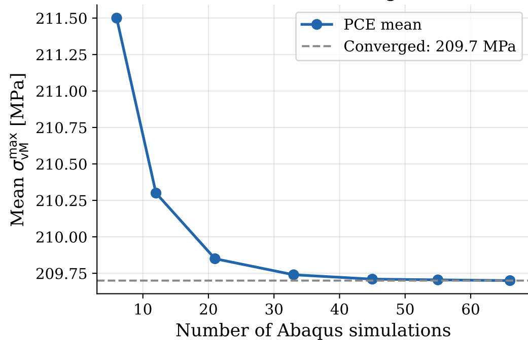
PCE Mean — Convergence
