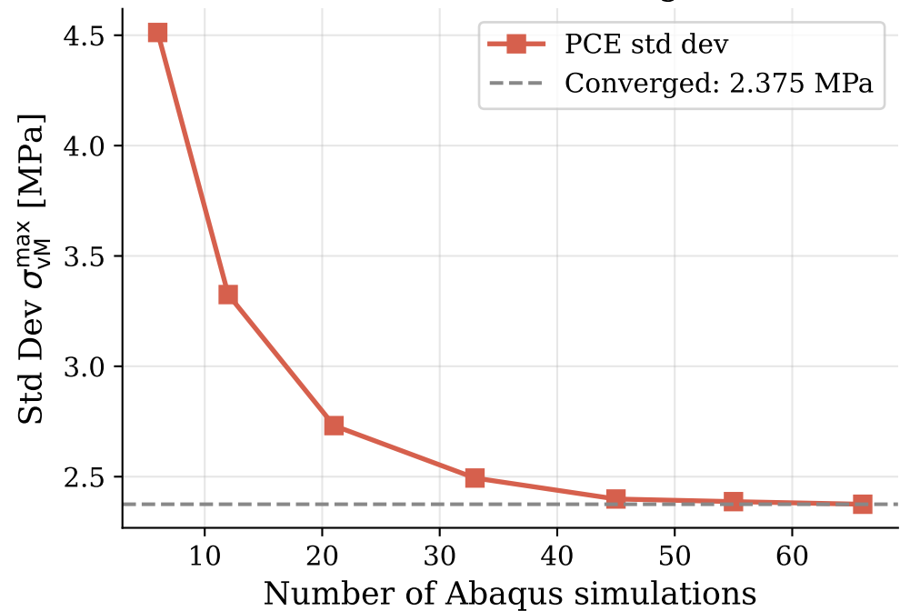
PCE Std Dev — Convergence
