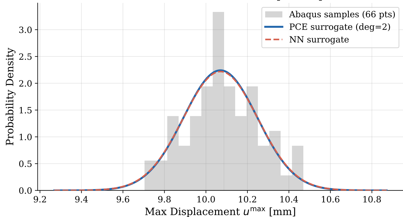
PDF of u^{\max} : PCE vs NN vs Abaqus samples
