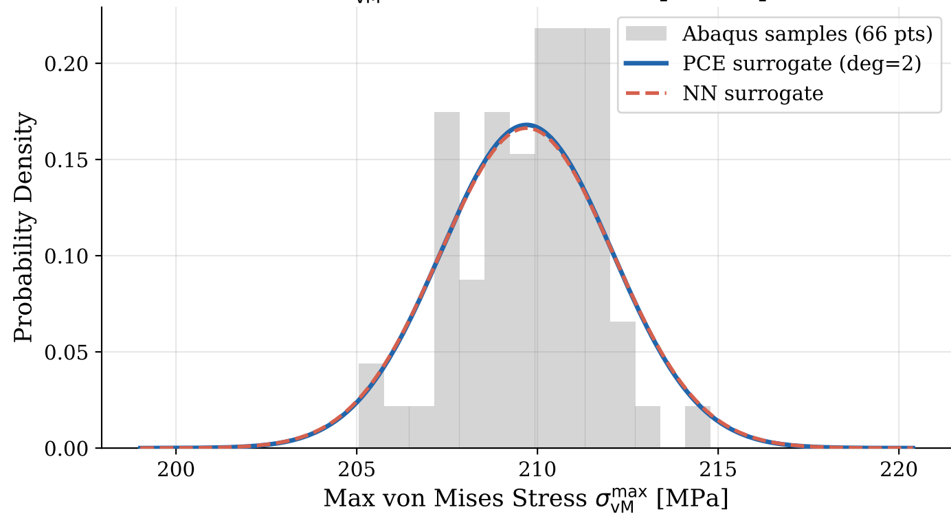
PDF of \sigma_{VM}^{max} : PCE vs NN vs Abaqus samples
