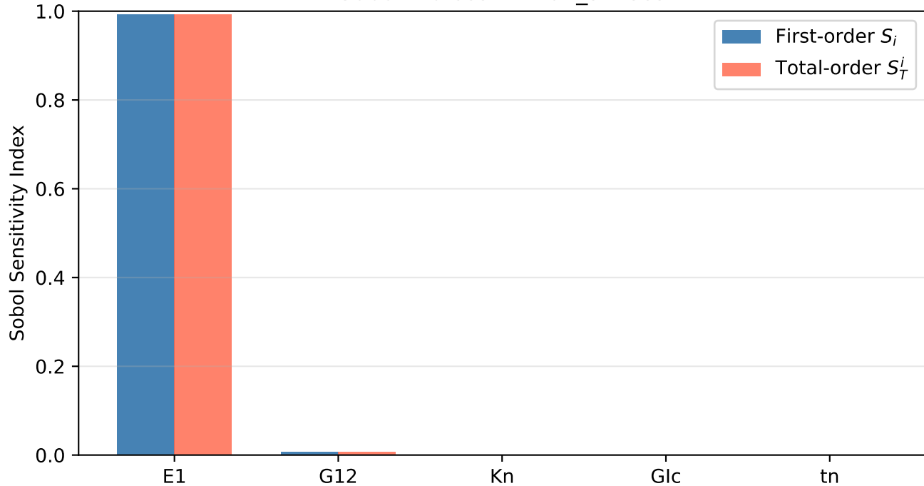
Sobol Indices — max_smises
