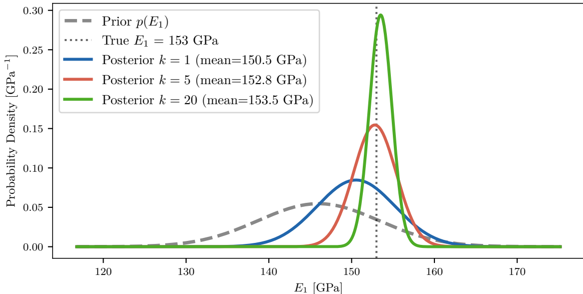
Bayesian Identification of E_1 : Prior vs Posterior
