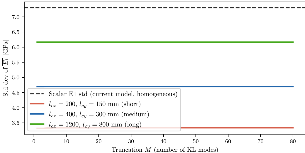
Spatial Mean \overline{E_1} Variability vs KL Truncation
