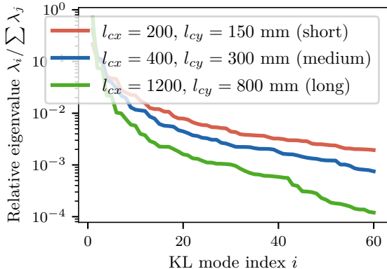
Eigenvalue Decay vs Correlation Length
