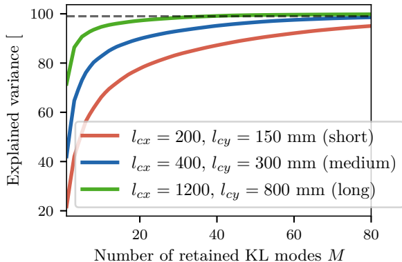
Explained Variance vs M
