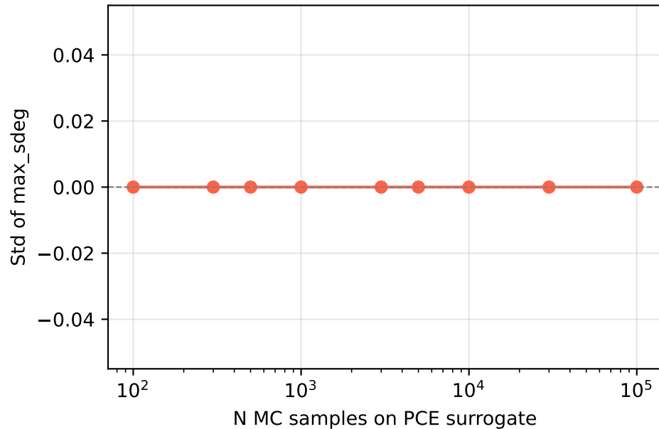
Convergence of Std
