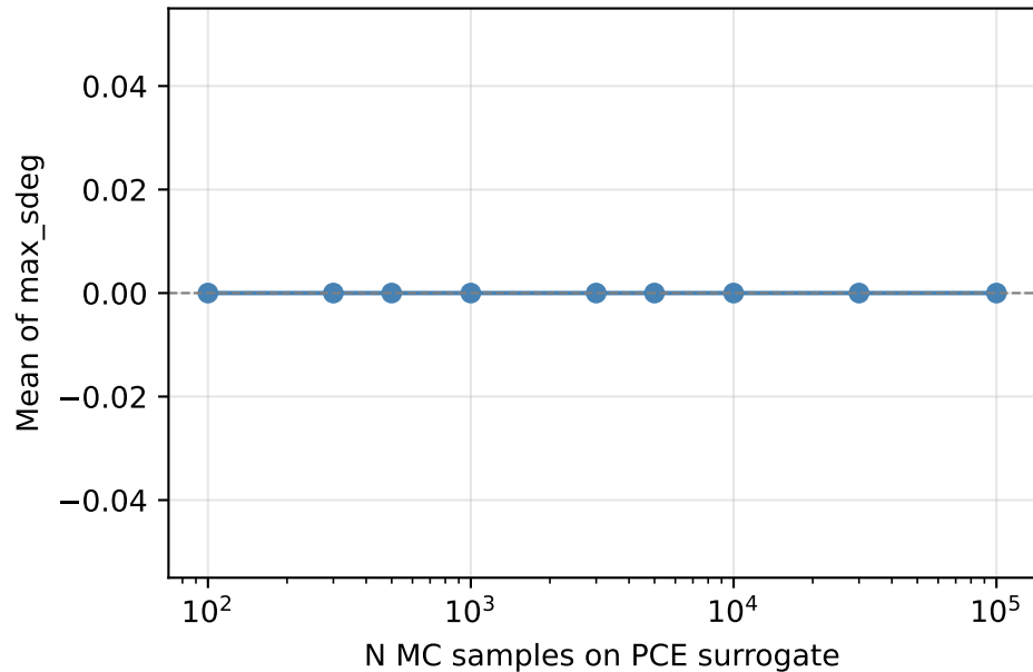
Convergence of Mean
