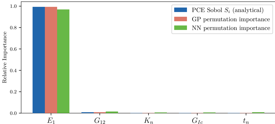
Sensitivity Analysis: PCE (Analytical) vs GP / NN (Permutation)
