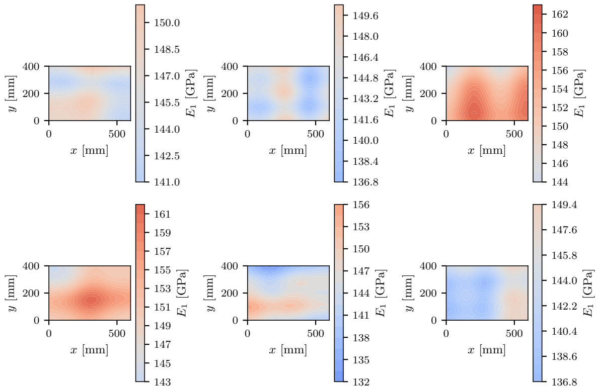
Sample Realisations of E_1(x, y) via KL Expansion ( M = 10 modes, 82.7% variance; l_{cx} = 400 mm)
