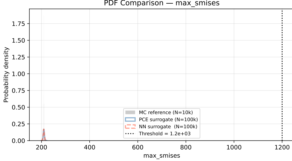
Figure 10: PDF comparison degree 3: max von Mises stress surrogate vs Abaqus samples.
