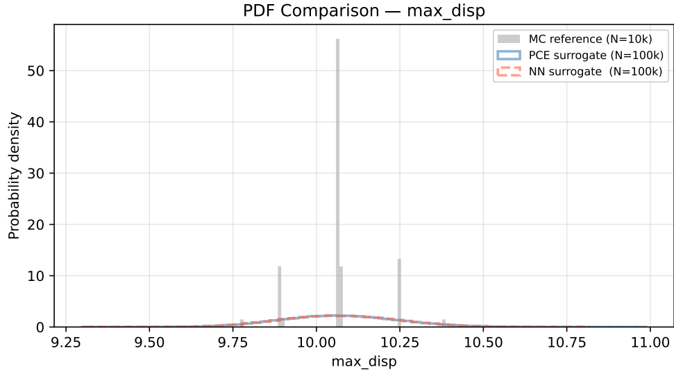
Figure 5: PDF of max displacement: PCE vs NN surrogate comparison. Degree 2.
