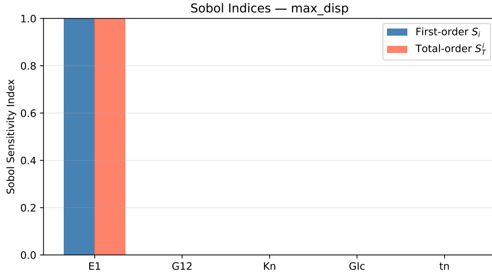
Figure 9: Sobol sensitivity indices for max displacement (degree 3). E_1 dominance is confirmed independently of polynomial degree.
