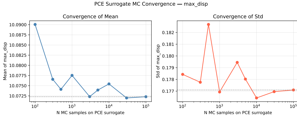
Figure 7: PCE convergence for max displacement (degree 2).
