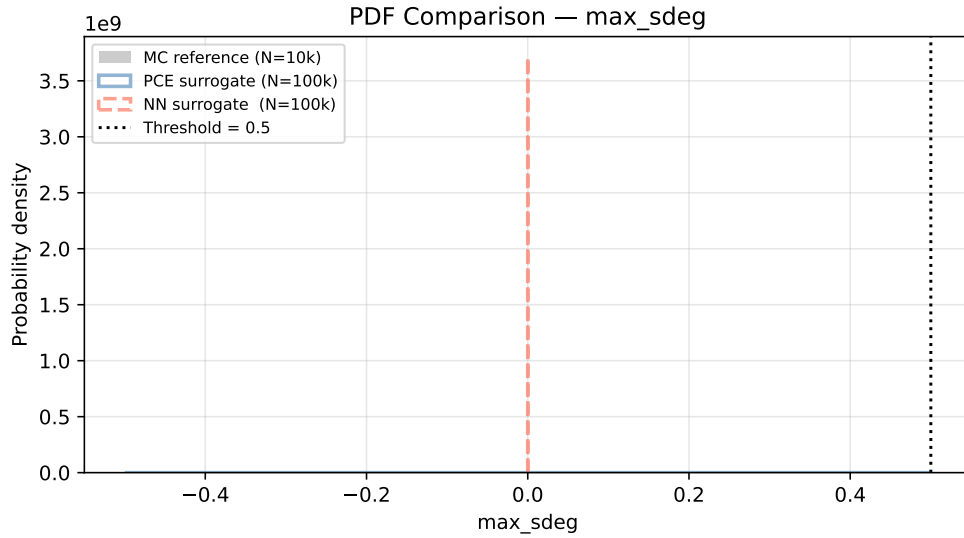
Figure 4: PDF of max scalar damage variable (SDEG): all 66 Abaqus samples return SDEG = 0 , confirming no cohesive damage initiation under any parameter realisation.
