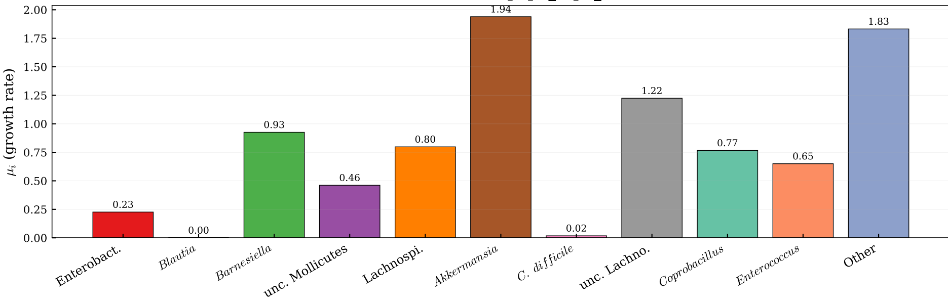
Growth rates — pop3_rep2_id6
