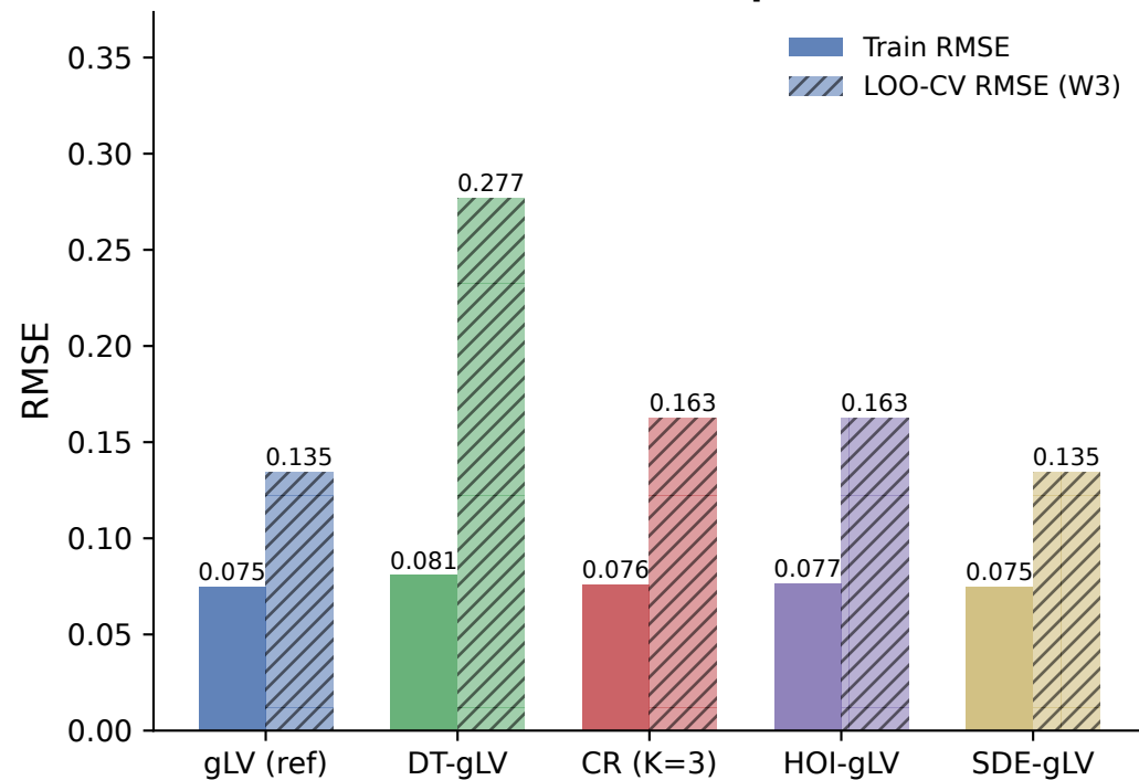
Train vs LOO-CV (W3 prediction)
