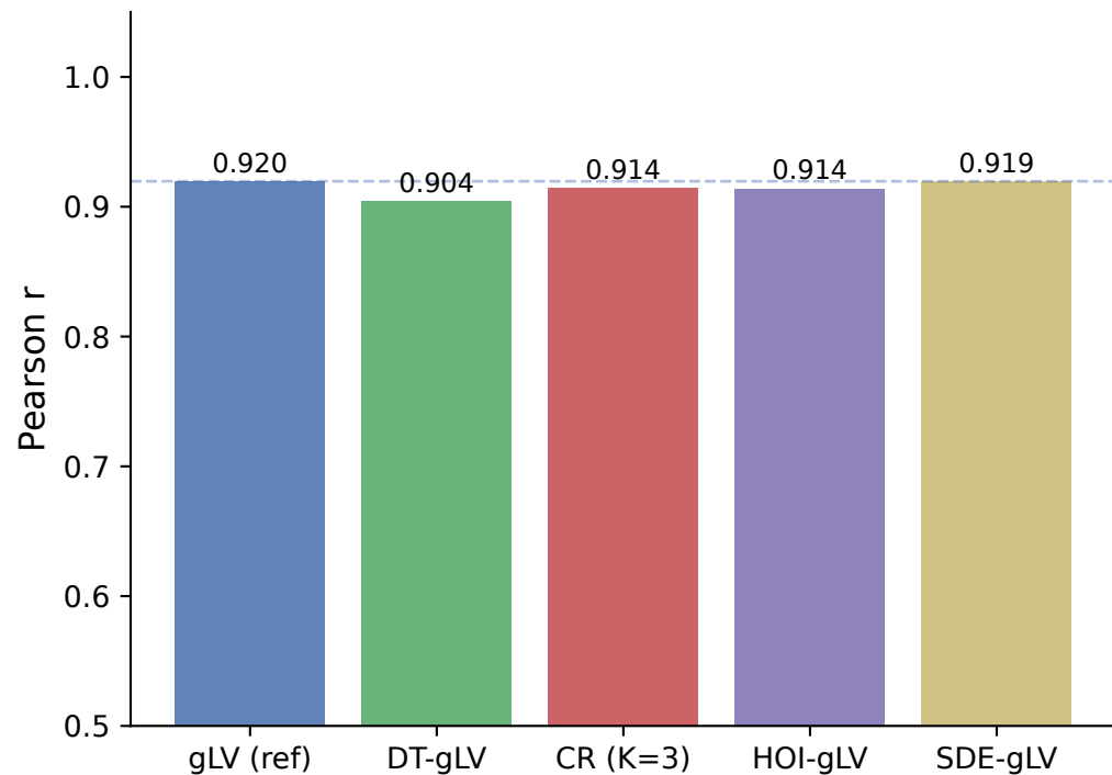
Prediction correlation (r)
