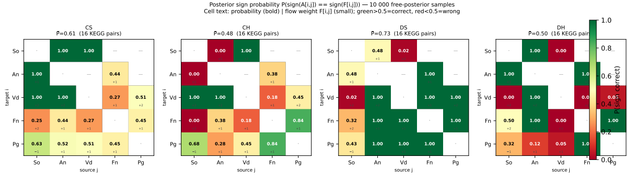
Figure 8: Posterior sign probability P_{ij} for each KEGG/eHOMD pair from 10 000 free-posterior samples. Each cell shows P_{ij} (bold) and the net-flow weight F_{ij} (small text). Green ( P > 0.5 ): free posterior supports the KEGG-predicted sign; red ( P < 0.5 ): data-driven sign opposes KEGG prediction; grey dashes: pair not in the KEGG/eHOMD network. The \text{An} \leftarrow \text{Vd} pair achieves P = 1.00 in all conditions; \text{So} \leftrightarrow \text{Vd} reverses from P = 1.00 (commensal) to P \approx 0 (dysbiotic).
