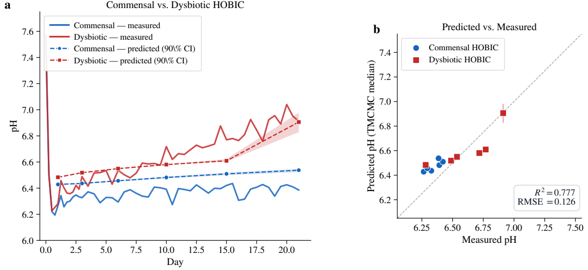
Figure 6: Independent pH validation. (a) Measured HOBIC pH time series (solid lines) overlaid with TMCMC posterior predictions (dashed lines, markers) and 90% credible intervals (shaded bands) for commensal (blue) and dysbiotic (red) conditions. (b) Scatter plot of TMCMC-predicted vs. measured pH at six time points ( t = 1, 3, 6, 10, 15, 21 days); vertical bars indicate 90% posterior CIs. Regression coefficients were fitted solely from experimental species fractions (LOO-CV, N = 90 ); pH data were not used in TMCMC calibration. R^2 = 0.778 , RMSE = 0.126 pH units ( N = 12 points, two conditions).
