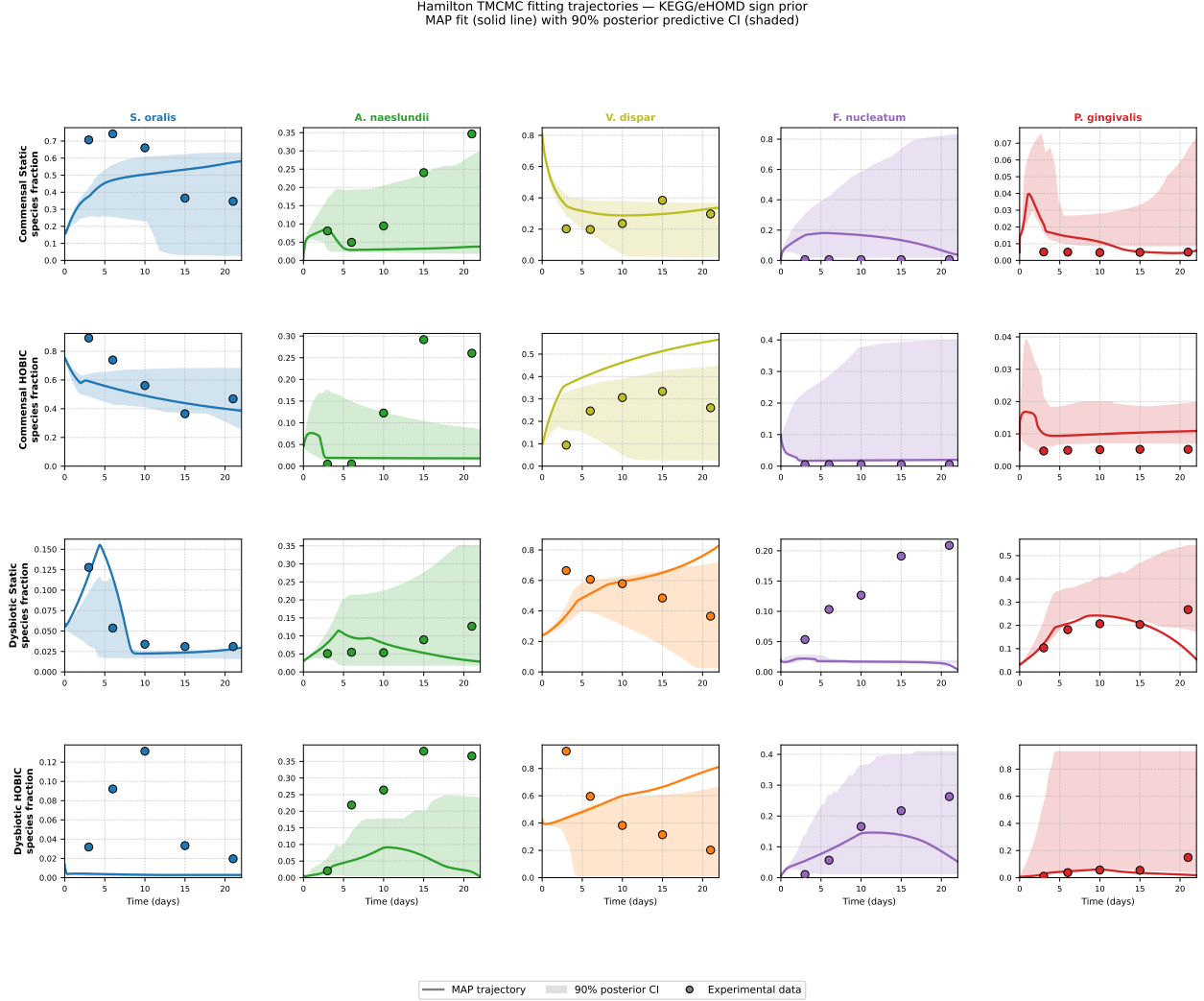
Figure 10: Posterior predictive trajectories for the Hamilton TMCMC runs with KEGG/eHOMD sign prior. Each panel shows one species (columns) in one condition (rows). Solid lines: MAP trajectory; shaded bands: 90 % posterior predictive CI from 80 TMCMC samples; circles: experimental data from Heine et al. [5]. The sign prior preserves data fit while biasing interaction signs toward metabolically plausible directions.
