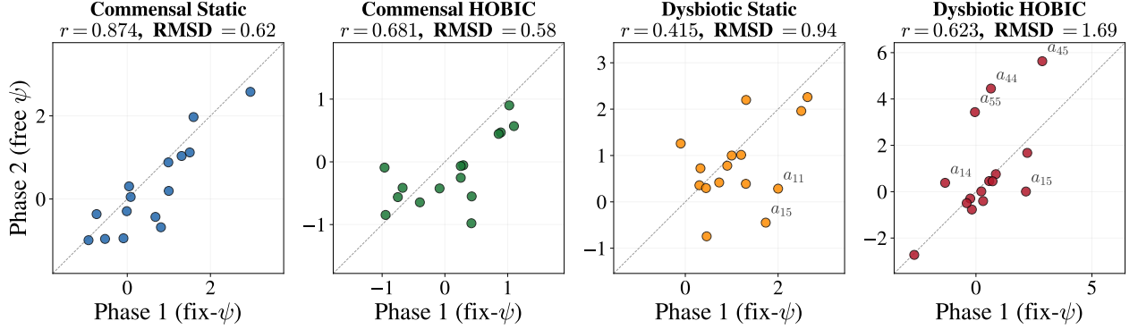
Figure 7: Phase 1 (fix- \psi ) vs. Phase 2 (free \psi ) MAP estimates. Each point is one of the 15 interaction parameters; dashed line: identity. CS ( r = 0.87 ) and CH ( r = 0.68 ) show good agreement, validating the fix- \psi approximation. Dysbiotic conditions (DS: r = 0.42 , DH: r = 0.62 ) exhibit systematic shifts in Pg-related parameters, confirming the necessity of Phase 2.
