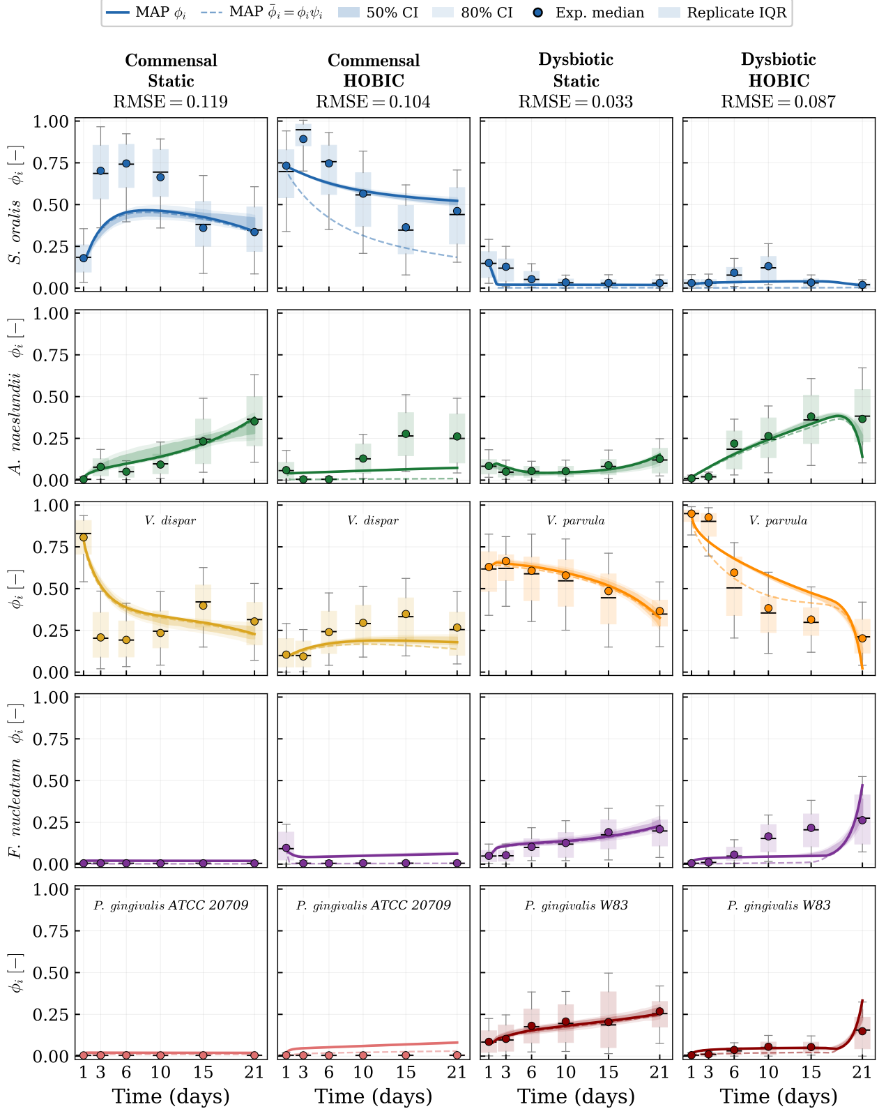
Figure 2: Posterior predictive fits of volume fraction \phi_i ( N_p = 10,000 ). Columns: four experimental conditions (CS, CH, DS, DH); rows: five species. Solid lines: MAP \phi_i trajectory; dashed lines: living fraction \bar{\phi}_i = \phi_i \psi_i . Shaded bands: 50% (dark) and 80% (light) credible intervals from 100 posterior samples. Circles: experimental median ( N = 8 replicates); box plots: inter-replicate variability (IQR). Note that P. gingivalis employs different strains: avirulent ATCC 20709 in commensal conditions and virulent W83 in dysbiotic conditions (indicated by colour).
