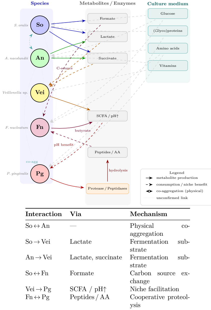
Figure 1: Metabolite-mediated interaction network based on Heine et al. [5] (Fig. 4C and metabolic profiles). Left: five model species (coloured circles) with full names. Centre: extracellular metabolites (grey boxes) and enzymatic activity (orange, Pg -derived proteases). Right: culture-medium substrates (teal). Solid arrows: metabolite production; dashed arrows: consumption or physiological benefit; dotted double-headed arrow: physical co-aggregation. Both So and An supply lactate and succinate to Vei, which ferments them to short-chain fatty acids (SCFA), raising local pH and promoting Pg growth. Pg-derived proteases hydrolyse (glyco)proteins into peptides and amino acids, fuelling Fn growth (cooperative Fn–Pg association). Grey dotted arrows between species: no confirmed metabolic pathway; all 20 interaction parameters are estimated freely—the posterior determines their magnitude.
