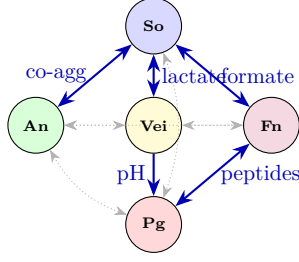
Fig. 1 Species interaction network (Heine et al. 2025). Solid: previously reported or biologically supported interactions considered in the interpretation of the model. Dotted grey: no reported pathway. All pairs are estimated with the same prior.
