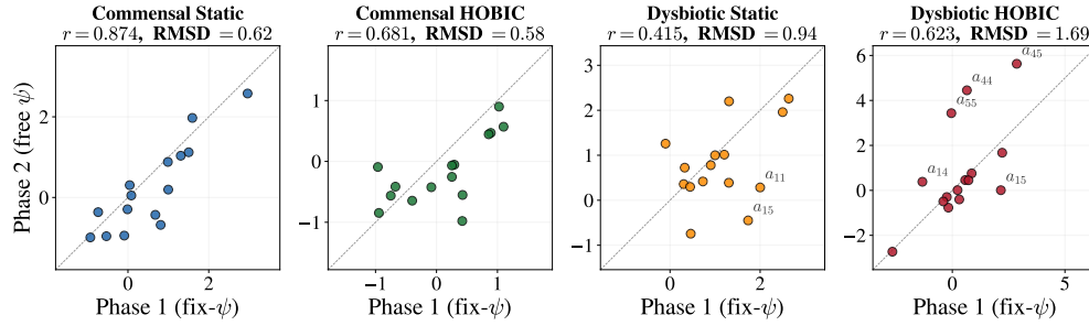
Fig. 6 Phase 1 (composition only) vs. Phase 2 (with viability and pH) MAP estimates. Each point is one of the 15 parameters; dashed line: identity. [update with the final runs]
