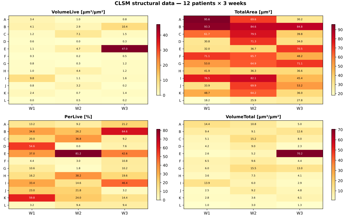
Figure 11: CLSM structural measurements for 12 patients \times 3 weeks. (a) VolumeLive [ \mu\text{m}^3 \mu\text{m}^{-2} ]; (b) TotalArea [ \mu\text{m}^2 ]; (c) PerLive [%]; (d) VolumeTotal. Patient I and J were excluded from the ODE analysis (no 16S data) but structural data are shown for completeness. Occupancy \tilde{\omega} used in Eq. (5) is derived from panels (a,b).
