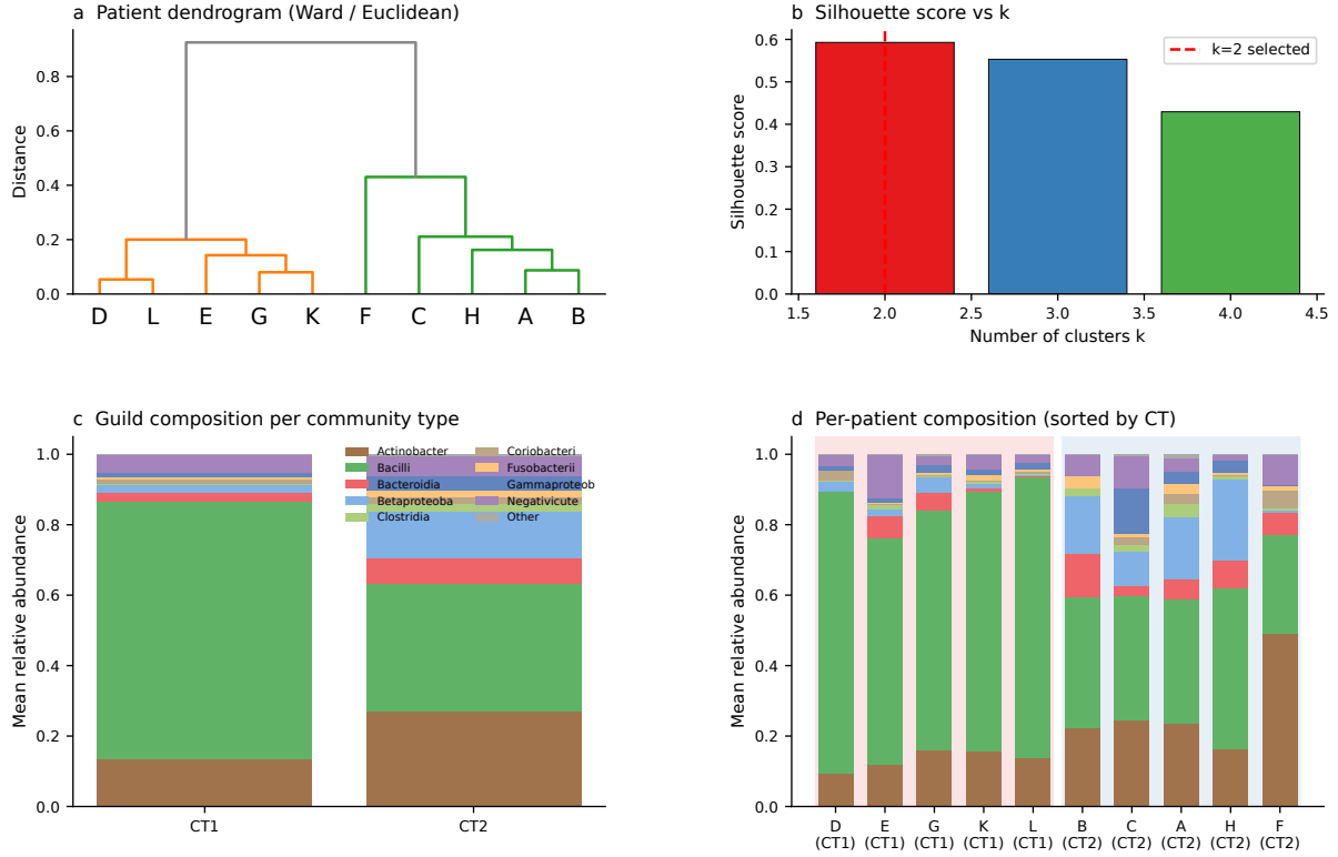
Figure 18: Community type analysis. (a) Ward dendrogram of 10 patients by mean 10-guild composition. (b) Silhouette scores; k = 2 selected. (c) Mean guild composition per CT. (d) Per-patient composition sorted by CT; background shading indicates CT assignment.
