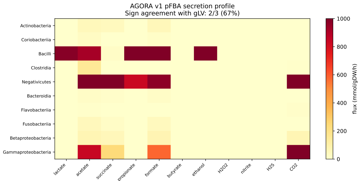
Figure 28: AGORA v1.03 pFBA secretion profiles for the 10 oral guilds under an oral-fluid medium. Each cell shows the net secretion flux ( \text{mmol gDW}^{-1} \text{h}^{-1} ) for a key metabolite class from parsimonious FBA on the AGORA v1.03 (With Mucins) SBML reconstruction of the guild representative organism. Carbon sources were capped at oral-fluid levels; vitamins and cofactors were left at model defaults to ensure feasible growth. Guild representatives: Actinomyces naeslundii (Actinobacteria), Atopobium parvulum (Coriobacteriia), Streptococcus gordonii (Bacilli), Parvimonas micra (Clostridia), Veillonella parvula Te3 (Negativicutes), Prevotella melaninogenica (Bacteroidia), Capnocytophaga sputigena (Flavobacteriia), Fusobacterium nucleatum (Fusobacteriia), Eikenella corrodens (Betaproteobacteria), Haemophilus parainfluenzae (Gammaproteobacteria). The strong lactate secretion by Bacilli ( Streptococcus ) and succinate secretion by Betaproteobacteria ( Eikenella ) and Bacteroidia ( Prevotella ) are consistent with the corresponding positive gLV entries.
