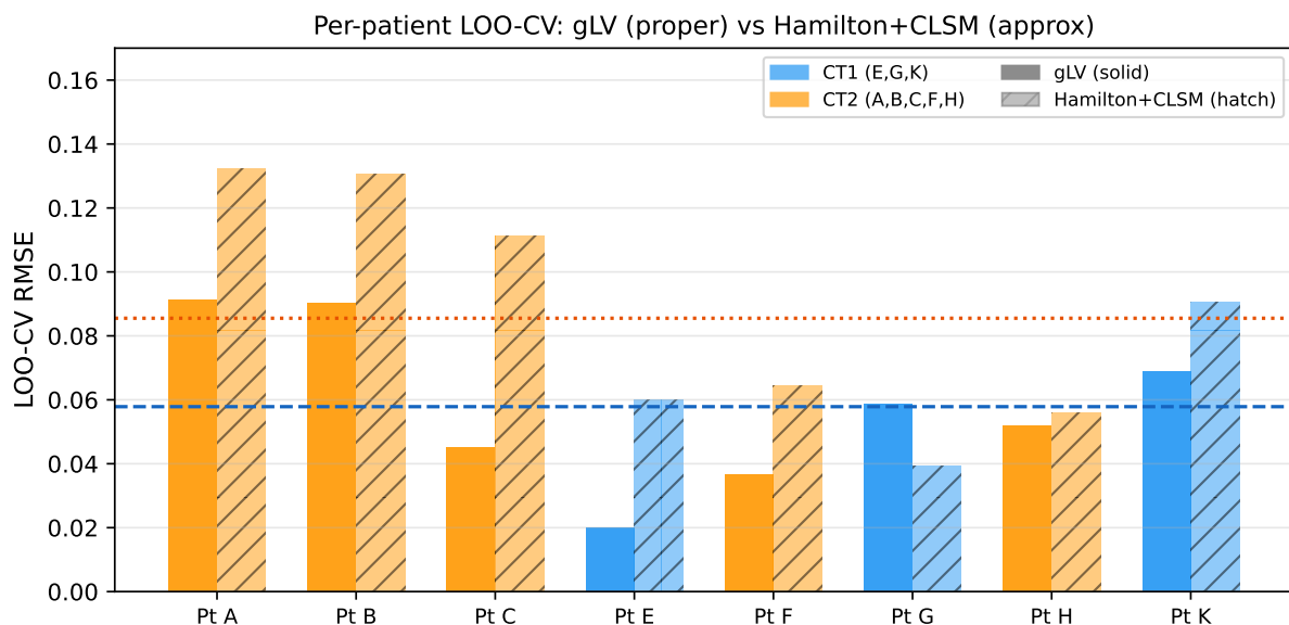
Figure 9: Per-patient LOO-CV RMSE comparison between gLV (solid bars, proper LOO: A re-fitted on 7 patients) and Hamilton+CLSM (hatched bars, approximate LOO: A fixed from full-cohort fit). Blue: CT1 patients (E, G, K); orange: CT2 patients (A, B, C, F, H). Horizontal lines: cohort means (gLV: 0.059; Hamilton: 0.086). CT2 patients consistently show higher LOO errors in both models (gLV CT2 = 0.064, CT1 = 0.051; Hamilton CT2 = 0.099, CT1 = 0.063), indicating that the more diverse CT2 community is harder to generalise from limited training data.
