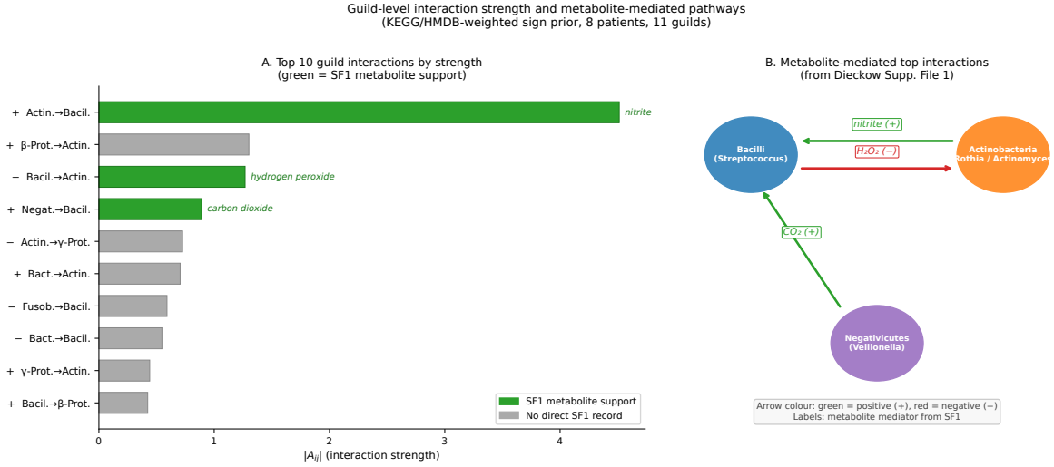
Figure 26: Guild interaction strength and metabolite-mediated pathways. A. Top 10 off-diagonal entries of the KEGG/HMDB-prior gLV A matrix ranked by |A_{ij}| (RMSE = 0.045, r = 0.963 , 8 patients, 11 guilds). Green bars indicate guild pairs for which at least one metabolite mediator is recorded in Dieckow Supp. File 1; grey bars indicate pairs lacking a direct SF1 annotation. Metabolite labels ( italic ) are shown for SF1-supported interactions. B. Schematic of the three dominant metabolite-mediated pathways recovered from SF1. Green arrows: positive (cross-feeding) interactions; red arrows: negative (inhibitory) interactions. The nitrite channel (Actinobacteria→Bacilli, A = +4.51 ), the H_2O_2 channel (Bacilli→Actinobacteria, A = -1.27 ), and the CO_2 cross-feeding (Negativicutes→Bacilli, A = +0.89 ) are each supported by primary literature on oral ecology.
