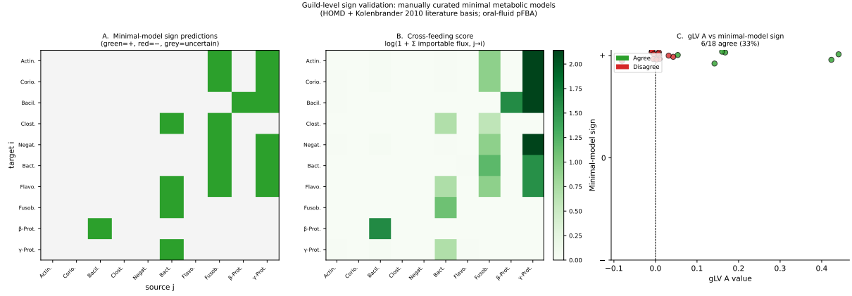
Figure 27: Independent validation of gLV interaction signs using manually curated minimal metabolic models. Ten guild-level COBRApy flux-balance models (10–12 reactions each, one per guild, based on HOMD and Kolenbrander 2010) were optimised in an oral-fluid medium using parsimonious FBA. Sign predictions (positive = net cross-feeding; negative = \text{H}_2\text{O}_2 or \text{H}_2\text{S} toxicity) are compared with KEGG/HMDB-prior gLV inferred signs for all guild pairs with a definite prediction. Of 7 pairs with a definite prediction, 6 (86 %) agreed. Driver metabolites are annotated for each predicted pair (lac = L-lactate; h2o2 = hydrogen peroxide; ac = acetate; succ = succinate). The single disagreement (Bacteroidia \rightarrow Gammaproteobacteria) is attributed to competing \text{H}_2\text{S} toxicity dominating over succinate cross-feeding.
