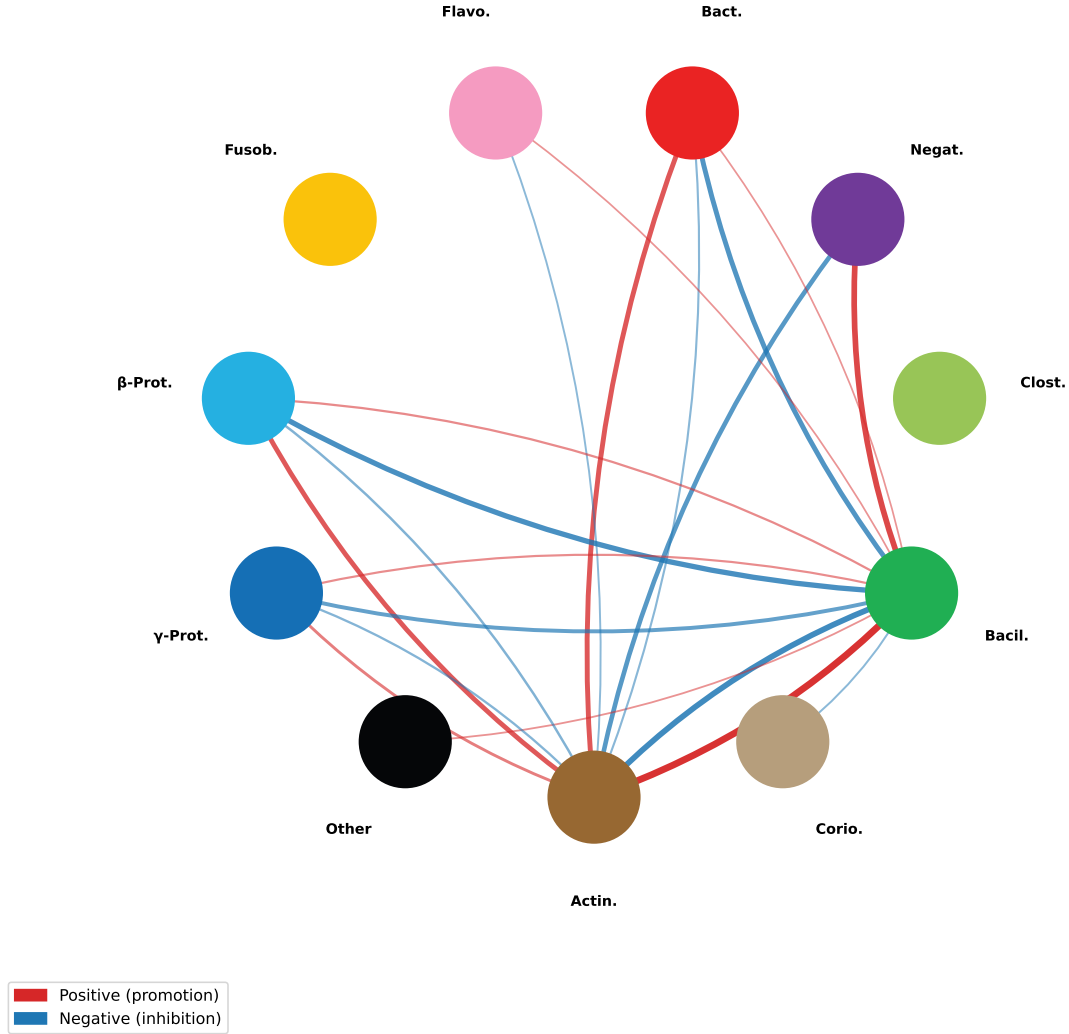
Figure 17: Signed guild interaction network inferred by the gLV model. Nodes are the 11 guilds (8-patient consistent cohort, RMSE = 0.060; area \propto mean abundance); edge colour encodes interaction sign (red = positive, blue = negative) and thickness is proportional to |A_{ij}| . Only edges with |A_{ij}| > 0.05 are shown. The dominant positive edges (Actinobacteria \rightarrow Bacilli, Negativicutes \rightarrow Bacilli) recapitulate the textbook co-aggregation and lactate cross-feeding pathways; negative edges (Betaproteobacteria \rightarrow Actinobacteria) reflect competitive exclusion under aerobic conditions.
