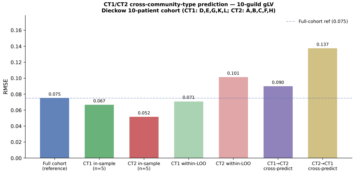
Figure 19: CT cross-community-type prediction. Bar heights show RMSE; solid bars: in-sample train RMSE; lighter bars (50% alpha): within-CT LOO-CV; solid bars at right: cross-CT prediction RMSE. CT1 \rightarrow CT2 prediction degrades by only 11% relative to within-CT2 LOO (0.090 vs. 0.101), while CT2 \rightarrow CT1 degrades by 93% (0.137 vs. 0.071), reflecting that CT2-specific Bacteroidia interactions are absent in CT1. Dashed line: full-cohort reference RMSE (0.075).
