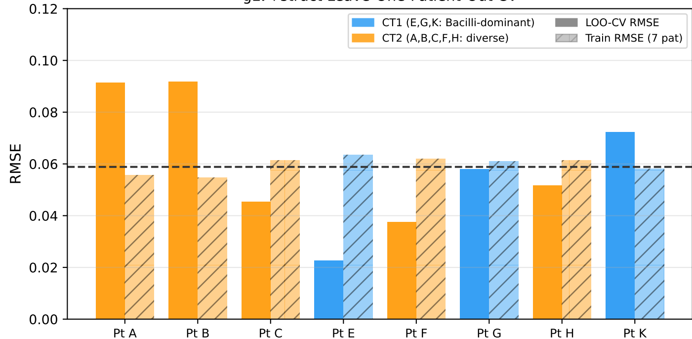
gLV+struct Leave-One-Patient-Out CV
