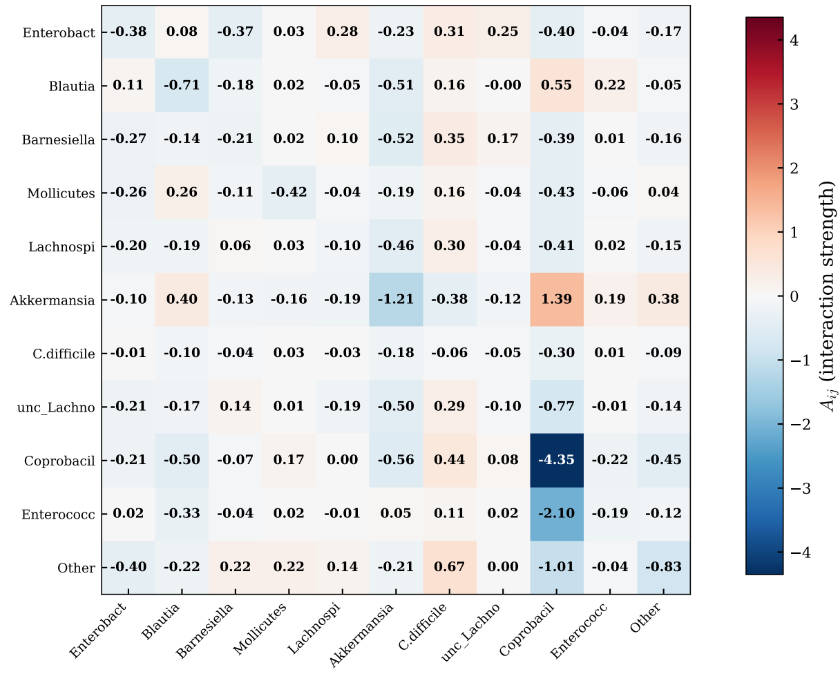
gLV (Stein 2013)
