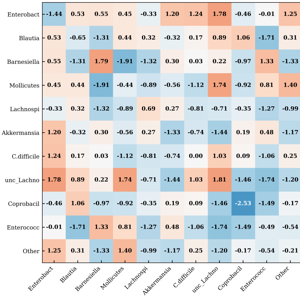
Hamilton ODE (this work)
