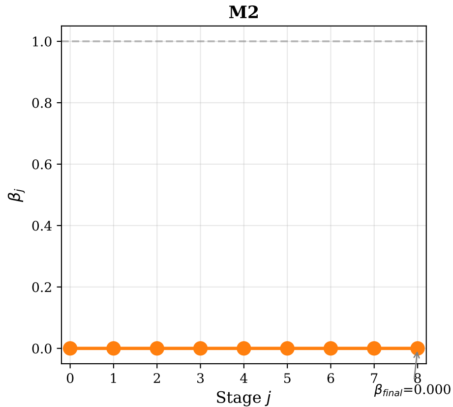
Figure 6: TCMC Tempering Schedule \beta_j
