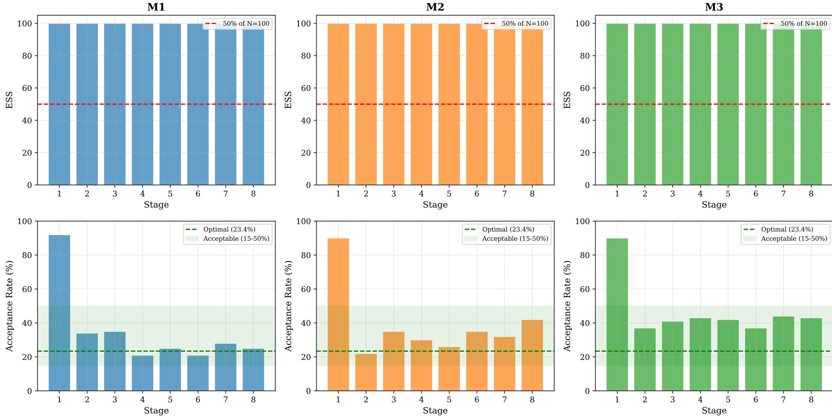
Figure 7: TCMC Convergence Diagnostics
