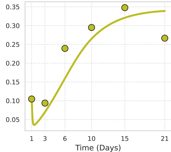
V. dispar
