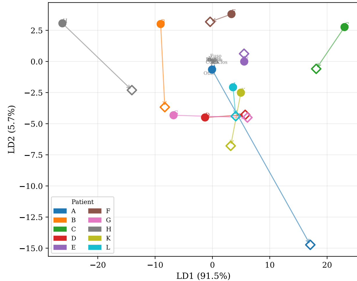
LDA — Week 2 (●=obs ◇=pred)
