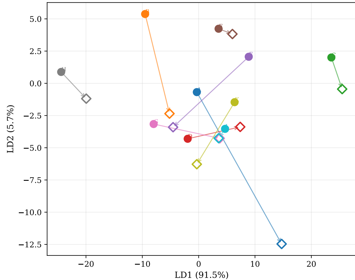
LDA — Week 3 (●=obs ◇=pred)
