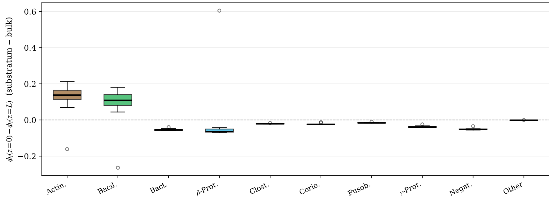
Substratum enrichment index across 10 LOO folds — gLV PDE (D_scale=1.0, u=0.005)
