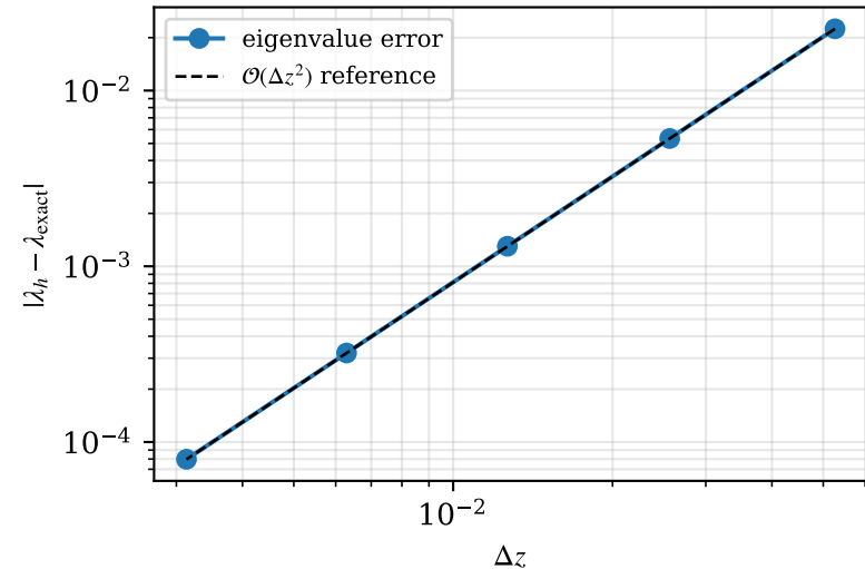
Diffusion stencil (interior+Neumann mode) slope 2.000
