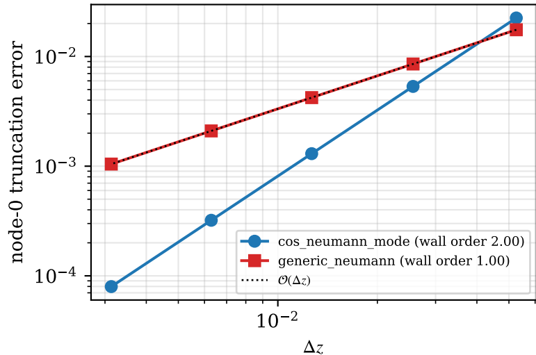
Ghost-node BOUNDARY order (2nd only for Neumann modes)
