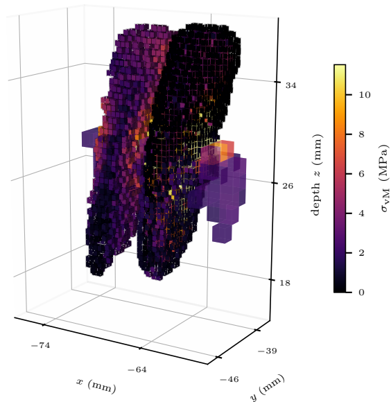
(B) occlusal von Mises (crestal-bone hot zone)
