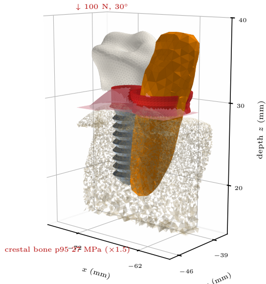
(B) restored: crown + gingiva (load at occlusal table)
