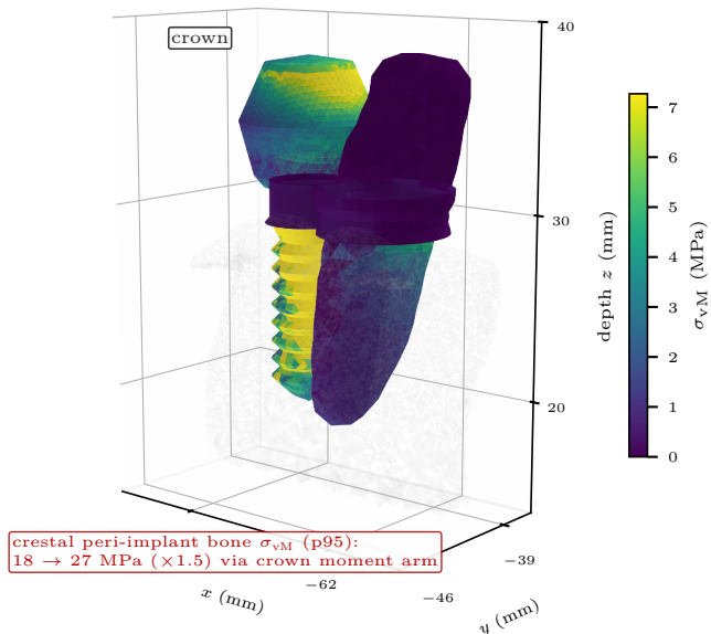
(B) occlusal von Mises \sigma_{vM} (crown included)
