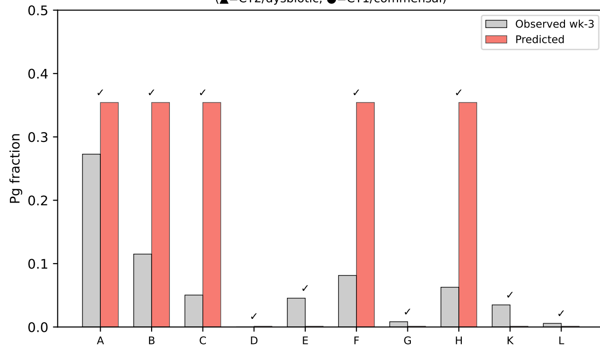
Plan B: attractor-only — Pg fraction (▲=CT2/dysbiotic, ●=CT1/commensal)
