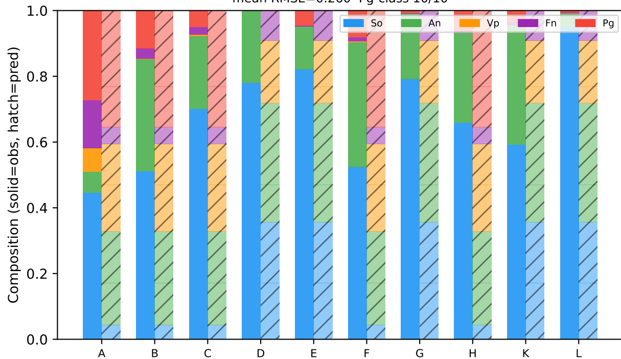
Plan B: attractor-only mean RMSE=0.260 Pg-class 10/10
