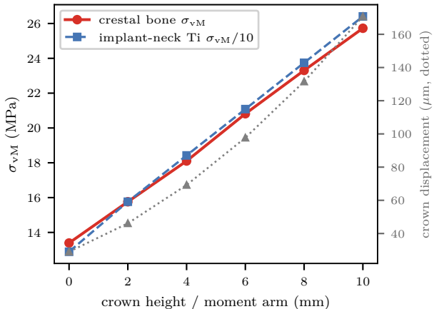
(A) crown HEIGHT dominates ( \times 1.9 over 0 \rightarrow 10 mm)
