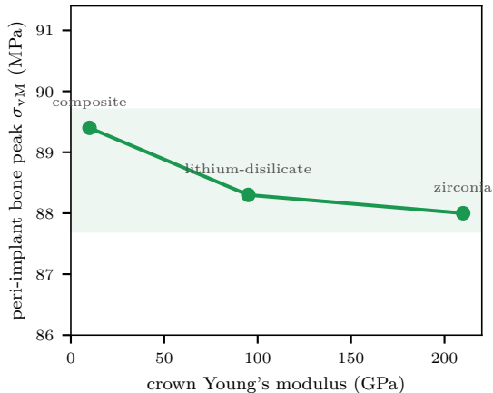
(B) crown MATERIAL is secondary ( < 2\% over 21\times )
