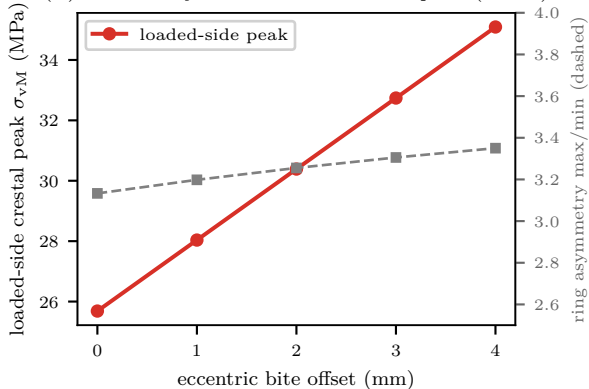
(B) eccentricity raises the loaded-side peak ( \times 1.37 )
